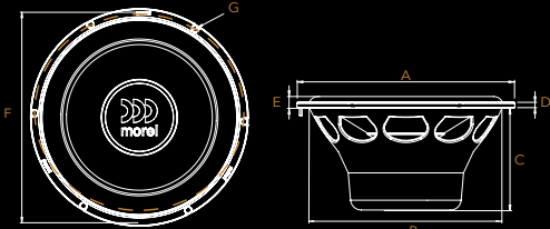
OVERALL DIMENSIONS
